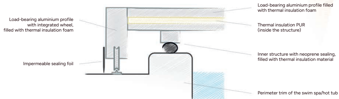
Thermal insulating PUR panel placed inside the cover structure, designed for swim spas and hot tubs
